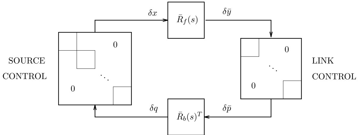
Figure 1: General congestion control structure.
