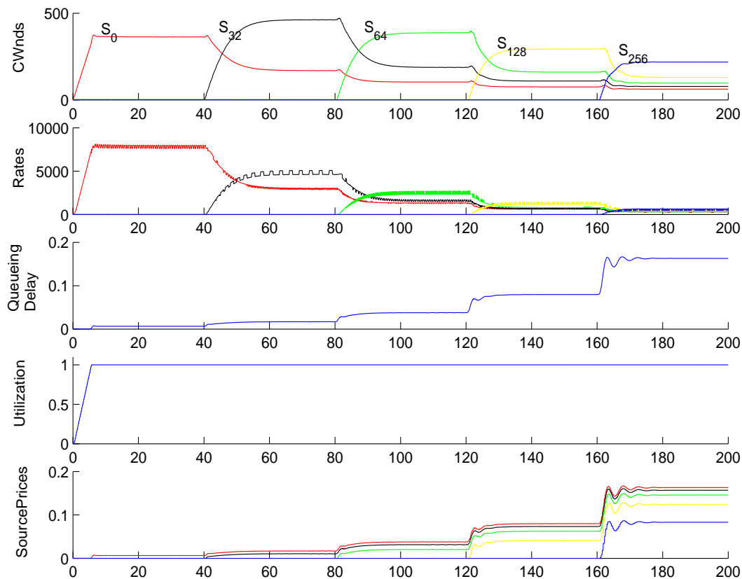
Figure 6: Dynamics of protocol based on queueing delay
