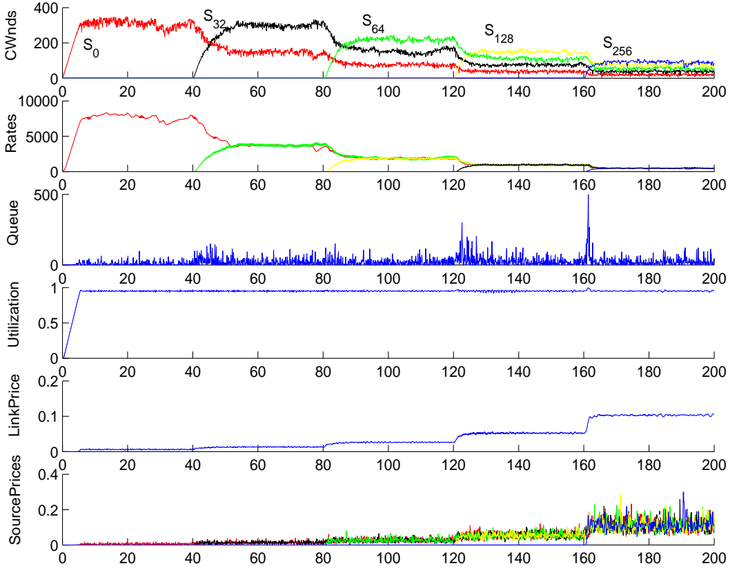
Figure 5: Dynamic Performance of the ECN-based Protocol
