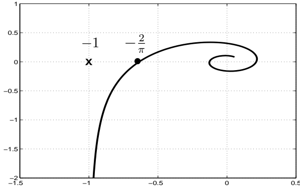
Figure 3: Nyquist plot \Gamma of e^{-j\theta}/j\theta .
