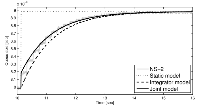
Fig. 2. Cross traffic. Both the joint model and the integrator model agree with the NS-2 simulation, but the static model leads significantly.
