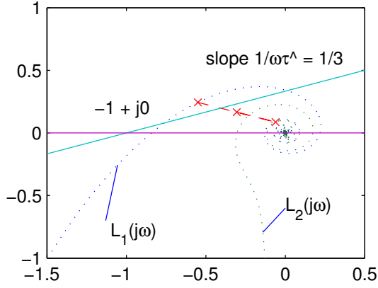
Fig. 4. An example of a line of slope 1/(\omega\hat{\tau}) which bounds L(j\omega) , denoted by the center cross. Note that the individual terms L_n(j\omega) , denoted by the individual crosses, are not all below this line.
