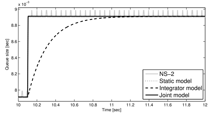
Fig. 1. Homogeneous sources. Both the joint model and the static model agree with the NS-2 simulation, but the integrator model lags significantly.
