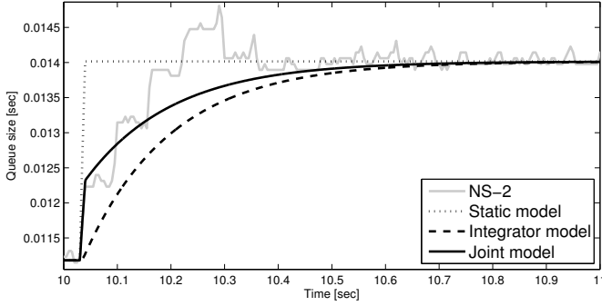
Fig. 3. Heterogeneous sources. The joint model captures both the initial jump and the protracted rise; the integrator model misses the former, while the static model misses the latter.
