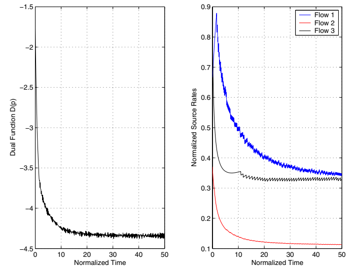
Fig. 5. The evolution of dual function and source rates with stepsize \gamma = 0.1 . The optimal flow rates are (1/3, 1/9, 1/3) .
