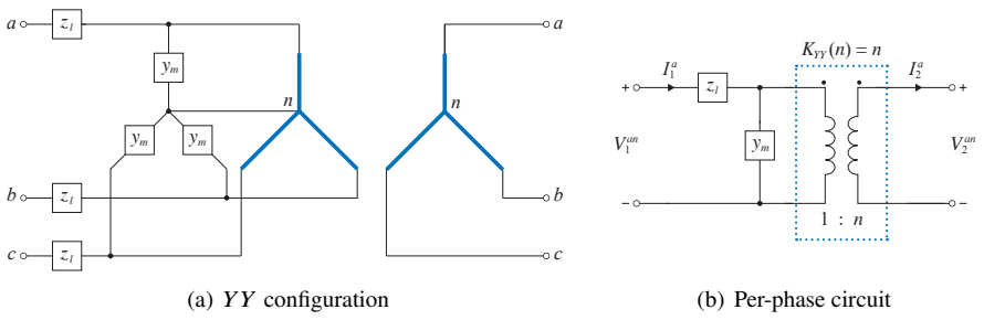
Figure 3.16 Three-phase transformers in YY configuration and its per-phase equivalent circuit.
