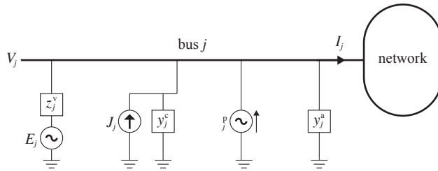
Figure 4.2 Multiple devices connected to the same bus.
