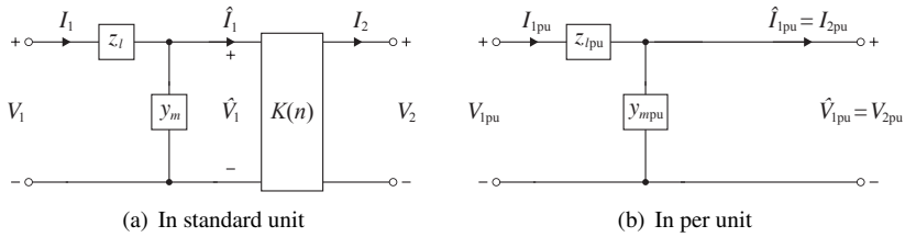
Figure 3.31 Per-phase equivalent circuit of balanced three-phase transformers with gain K(n) .
