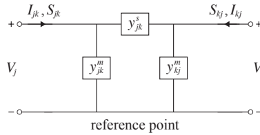
Figure 4.3 \Pi -circuit model of a single-phase branch.
