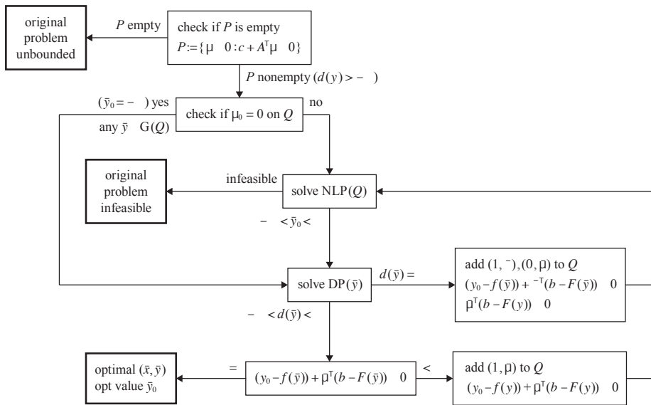
Figure 8.18 Benders decomposition.
