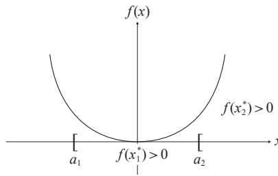
Figure 8.5 Example 8.6: \min_{x \geq a} x^2 . If a \leq 0 then the unique minimizer is x_1^* = 0 where f'(x^*) = 0 . If a > 0 then the unique minimizer is x_2^* = a where f'(x^*) > 0 .
