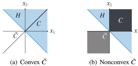
Figure 8.9 Example 8.7. (a) When \alpha = 1/2 , \tilde{C} = \{x : x_1 = x_2\} is convex. (b) When \alpha = 1 , \tilde{C} = \{x : x \geq 0\} \cup \{x : x \leq 0\} is nonconvex. In both cases C = \tilde{C} \cap H is convex.
