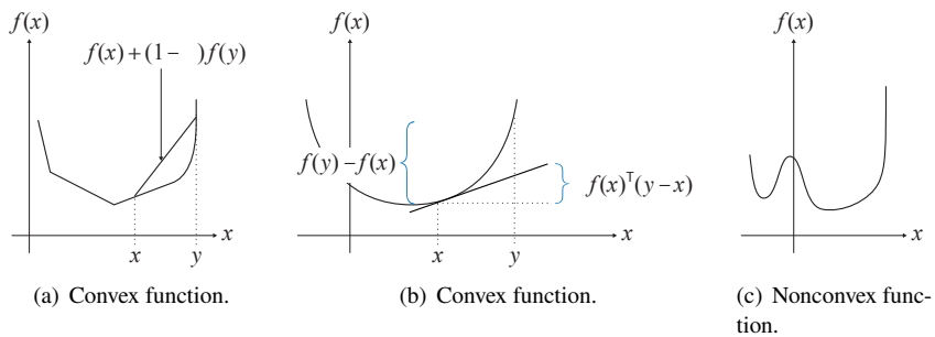
Figure 8.2 (a) The straight line connecting f(x) and f(y) lies above a convex f . (b) The linear approximation of a differentiable convex function f lies below f .
