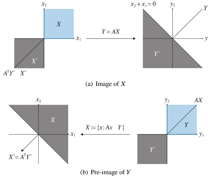
Figure 12.8 Example 12.4. Since A is singular, (a) A^\top Y^\circ \subsetneq X^\circ ; (b) A^\top Y^\circ = X^\circ ; moreover A^\top N_Y(\bar{y}) = N_X(\bar{x}) .
