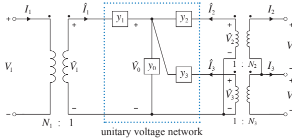
Figure 3.11 Single-phase split-phase transformer.
