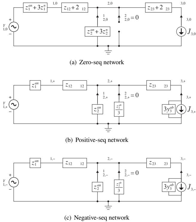
Figure 16.12 Example 16.14: Circuit models of sequence networks.
