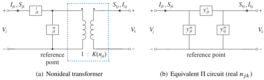
Figure 4.4 Single-phase transformer.
