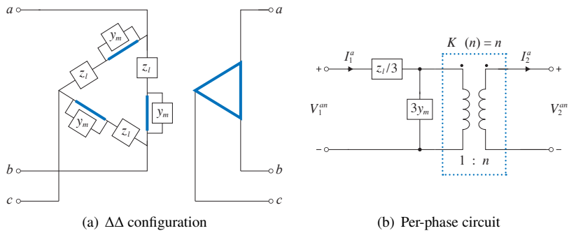
Figure 3.17 Three-phase transformers in \Delta\Delta configuration and its per-phase equivalent circuit.
