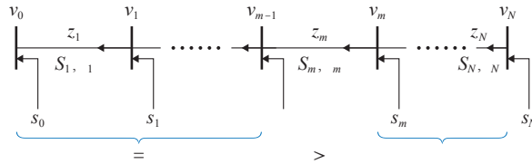
Figure 11.4 Linear network and notations. Line m in the proof is the line closest to bus 0 where the inequality in (11.27) is strict, i.e., (11.27) holds with equality at lines j = 1, \dots, m - 1 , strict inequality at line m , and inequality at lines j = m + 1, \dots, N .
