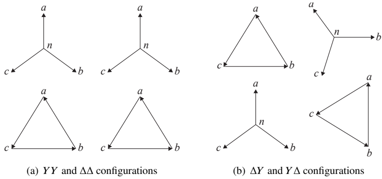
Figure 3.15 Compact representation of ideal three-phase transformers in (a) YY, ΔΔ configurations and (b) ΔY, YΔ configurations. For instance, in the YY configuration, the vertical arrow represents the vector V^{an} in the complex plane. The arrow from b to a (not shown) represents the vector V^{ab} . The parallel lines in the diagram indicate corresponding primary and secondary windings.
