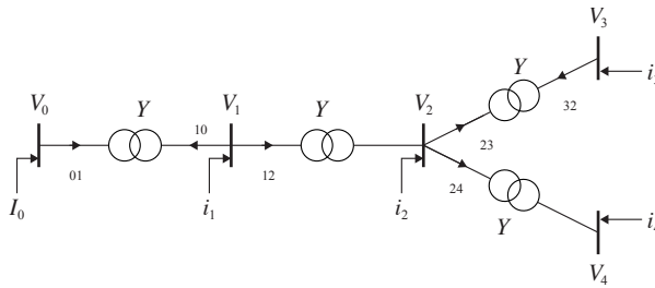
Figure 15.20 Radial network in Exercise 15.17.
