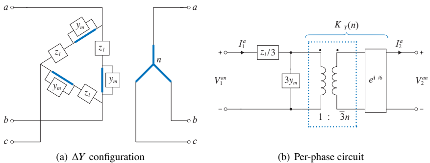
Figure 3.18 Three-phase transformers in \Delta Y configuration and its per-phase equivalent circuit.
