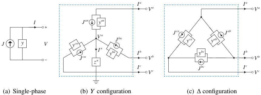
Figure 14.8 Comparison of single-phase and three-phase current sources.
