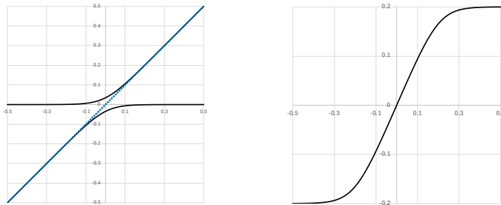
(a) f^\epsilon(x) : upper curve, g^\epsilon(x) : lower curve, y = x : dotted (b) h^\epsilon(x)
