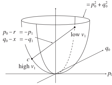
Figure 11.2 The nonconvex feasible set for a two-bus network without constraint consists of the (two) points of intersection of a line and a convex surface (without the interior). SOCP relaxation includes the interior and enlarges the feasible set to the line segment joining these two points. If the cost function C is increasing in \ell or (p_0, q_0) then the optimal point over the SOCP feasible set (line segment) is point c , and hence the relaxation is exact.
