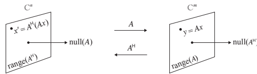
(a) Orthogonal decomposition of \mathbb{C}^n and \mathbb{C}^m
