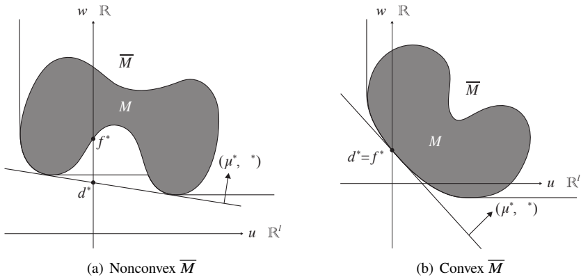
Figure 12.16 The (u, w) space: M := (h(X'), f(X')) := \{(h(x), f(x)) : x \in \text{dom}(f) \cap X'\} and its positive extension \overline{M} .
