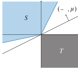
Figure 13.1 S-lemma: S, T and their separation.
