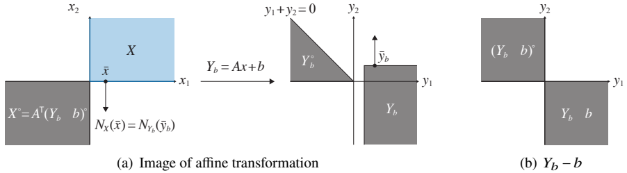
Figure 12.9 Example 12.5: while X is a cone, Y_b is not. X^\circ = A^\top(Y_b - b)^\circ and N_X(\bar{x}) = A^\top N_{Y_b}(\bar{y}_b) because A is nonsingular (Corollary 12.9).
