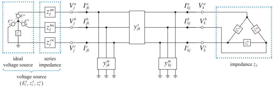
Figure 15.3 A voltage source connected to an impedance load through a three-phase line.
