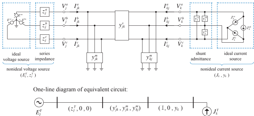
Figure 15.6 A voltage source connected to a current source through a three-phase line.
