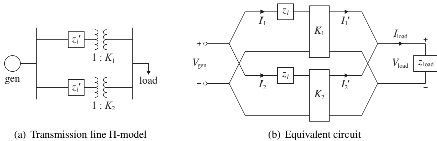
Figure 3.30 Two buses connected in a loop with two parallel transformers.
