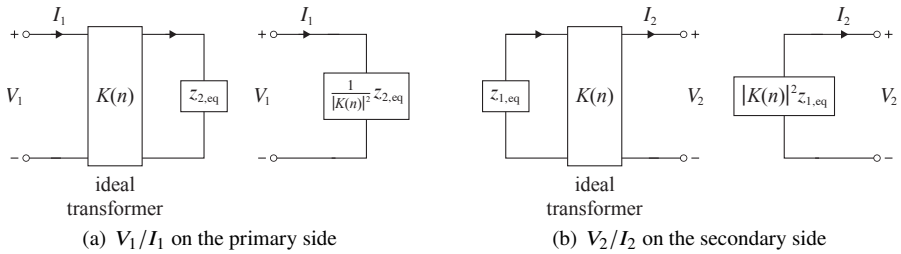
Figure 3.25 Driving-point impedances.
