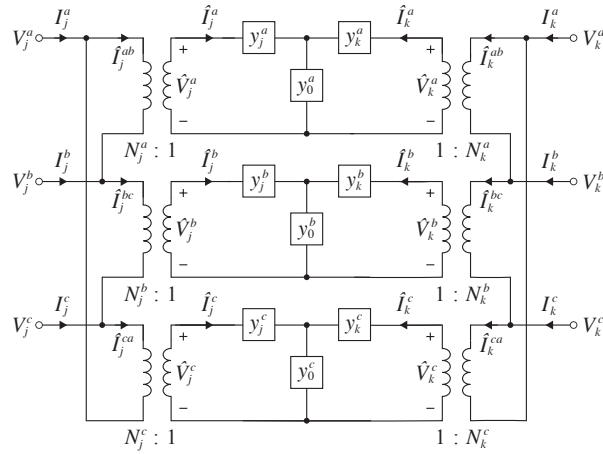
(b) \Delta\Delta configuration
