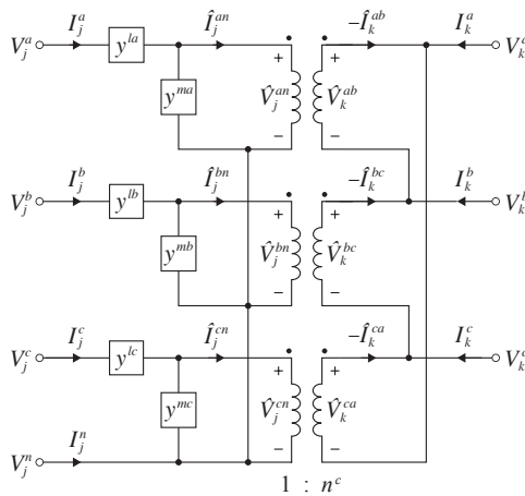
Figure 15.14 Y\Delta -configured transformer.
