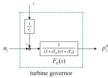
Figure 6.2 Block diagram in Laplace domain of the turbine-governor dynamic (6.14).
